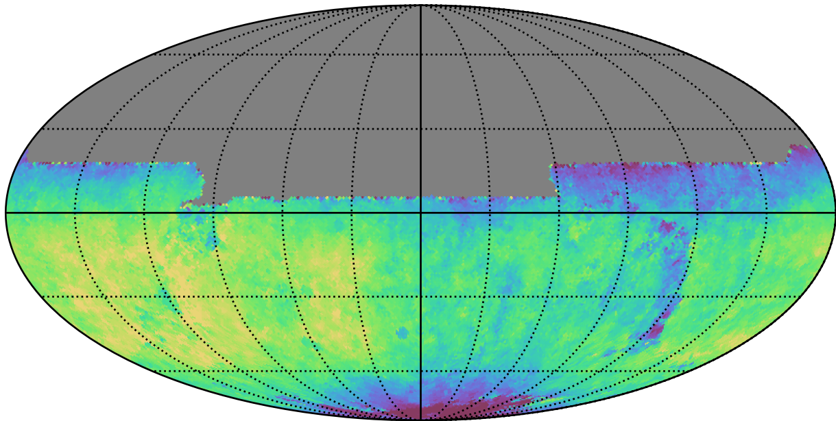
noroll_mjdp0_v3.4_10yrs All sky y band: Median saturation_mag
