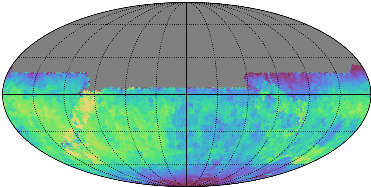
noroll_mjdp0_v3.4_10yrs All sky u band: Median saturation_mag
