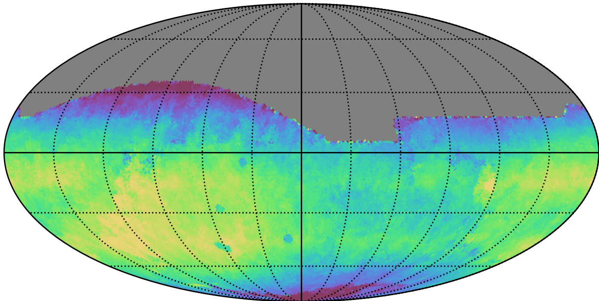
noroll_mjdp0_v3.4_10yrs All sky r band: Median saturation_mag
