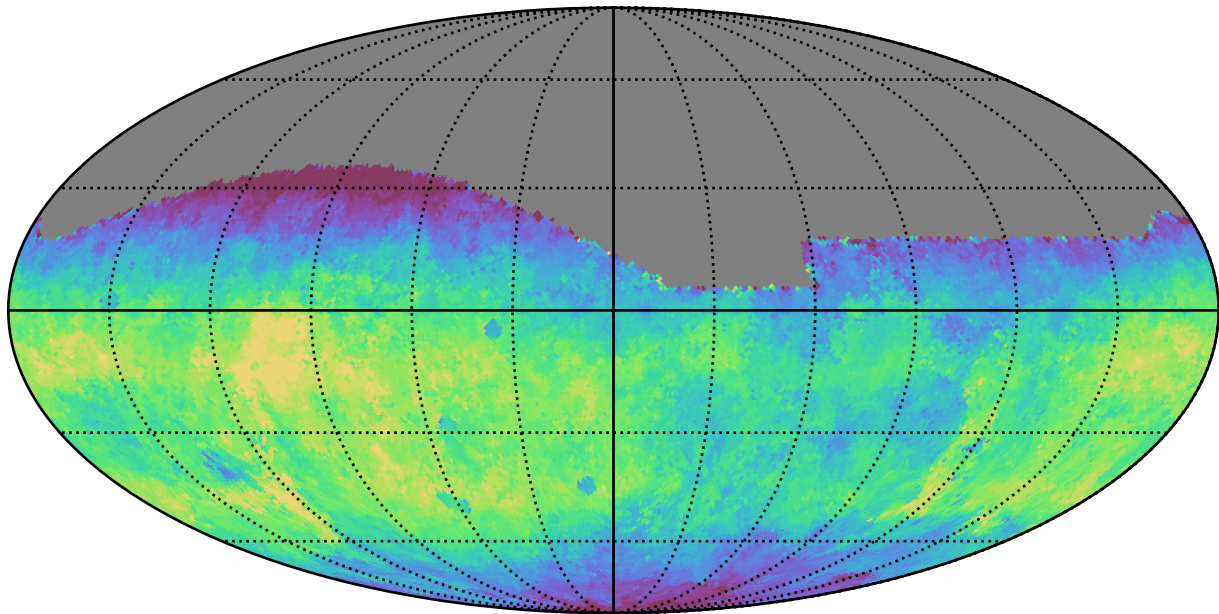
noroll_mjdp0_v3.4_10yrs All sky g band: Median saturation_mag
