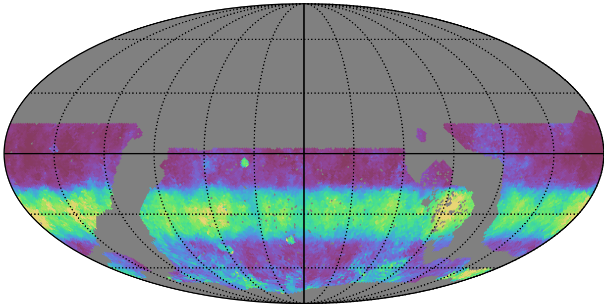
noroll_mjdp0_v3.4_10yrs WFD g band: Median normairmass
