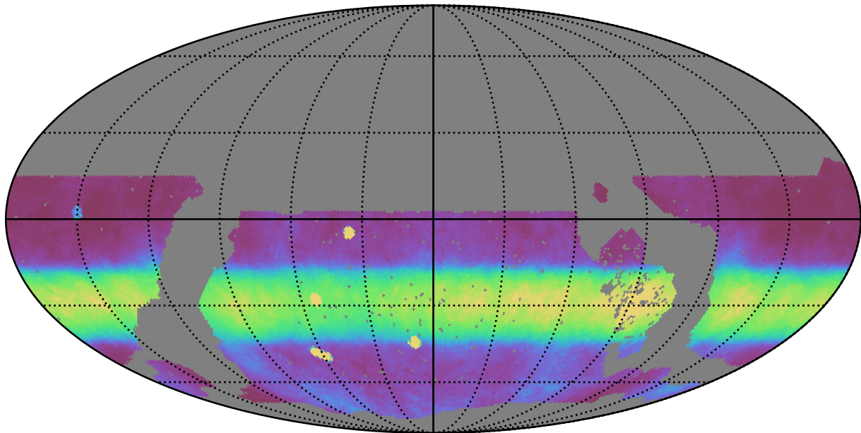
noroll_mjdp0_v3.4_10yrs WFD all bands: Median normairmass
