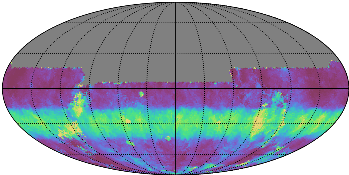
noroll_mjdp0_v3.4_10yrs All sky u band: Median normairmass
