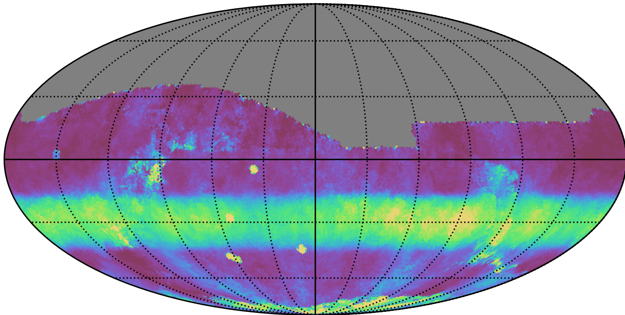
noroll_mjdp0_v3.4_10yrs All sky r band: Median normairmass
