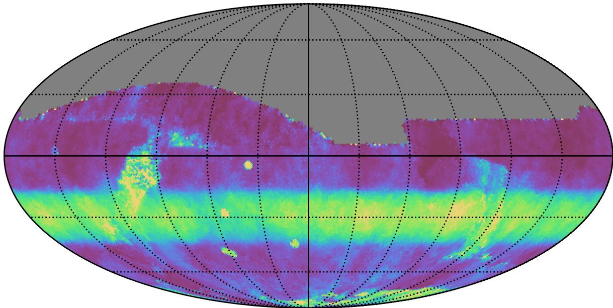
noroll_mjdp0_v3.4_10yrs All sky i band: Median normairmass
