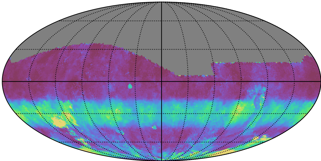
noroll_mjdp0_v3.4_10yrs All sky g band: Median normairmass
