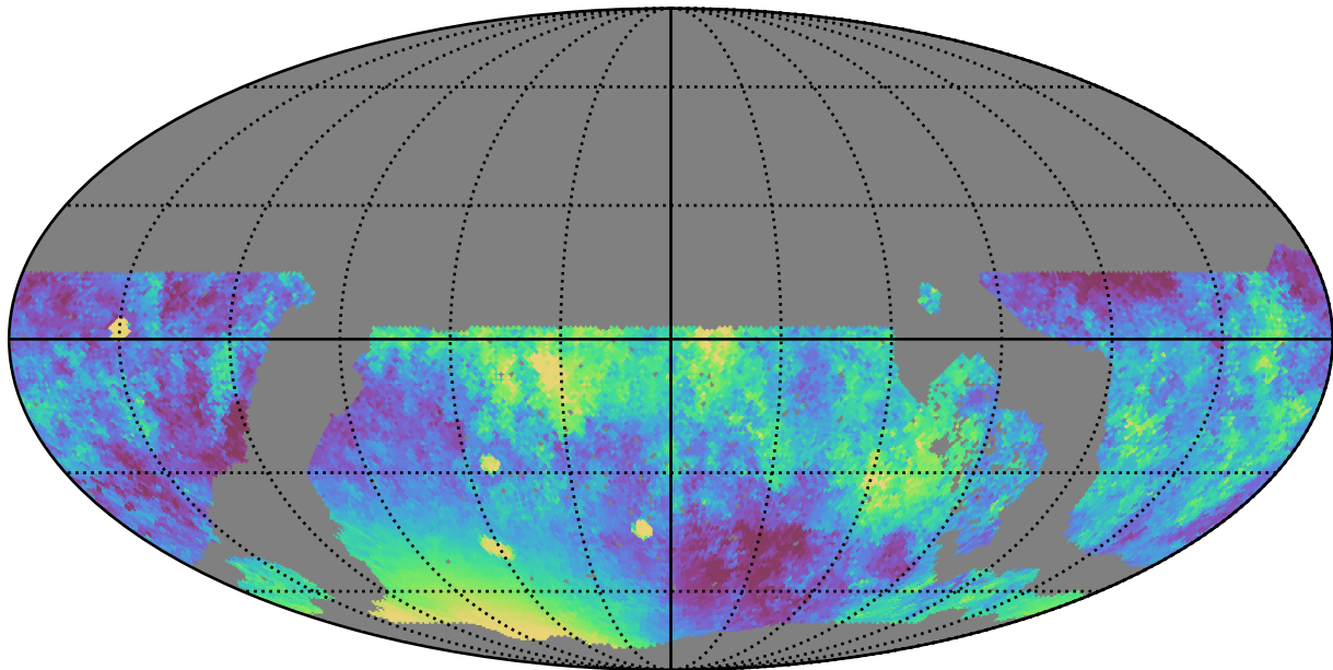
noroll_mjdp0_v3.4_10yrs WFD z band: Median moonDistance
