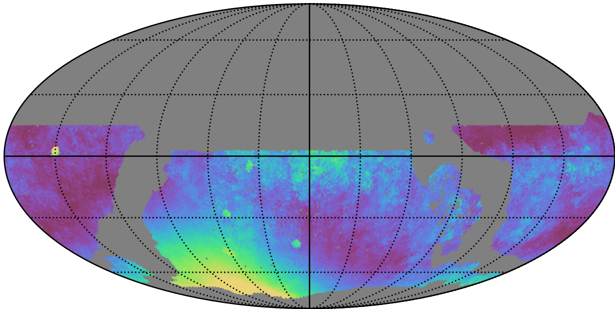
noroll_mjdp0_v3.4_10yrs WFD y band: Median moonDistance
