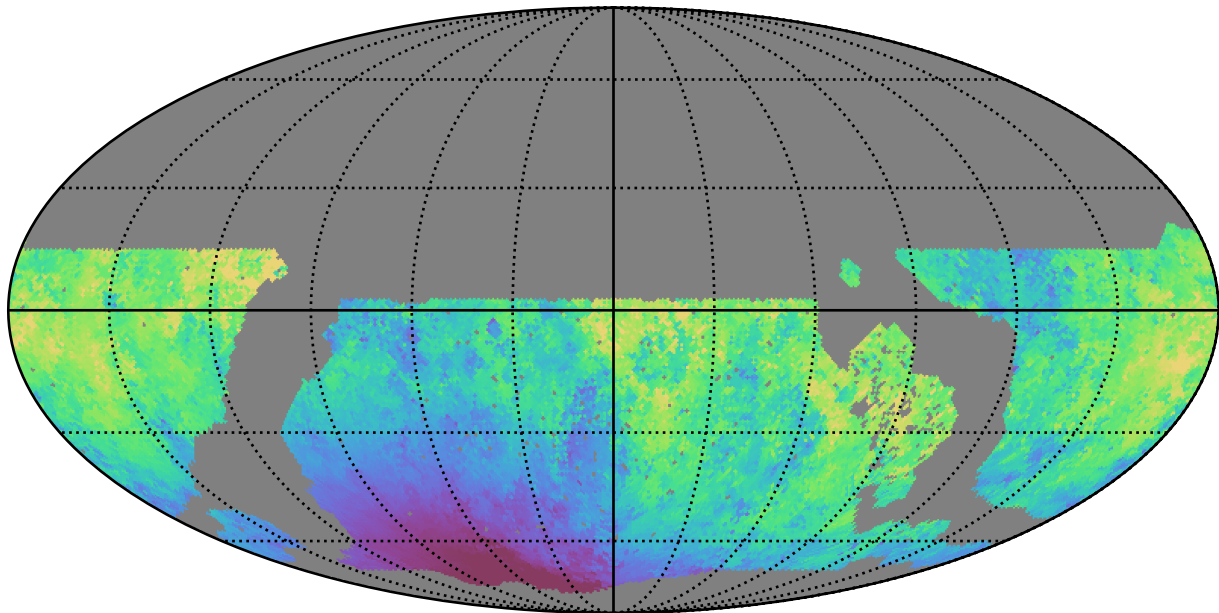
noroll_mjdp0_v3.4_10yrs WFD u band: Median moonDistance
