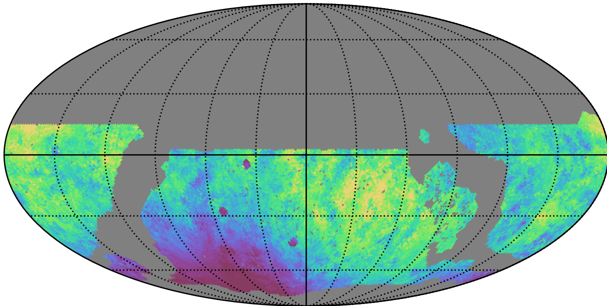
noroll_mjdp0_v3.4_10yrs WFD r band: Median moonDistance
