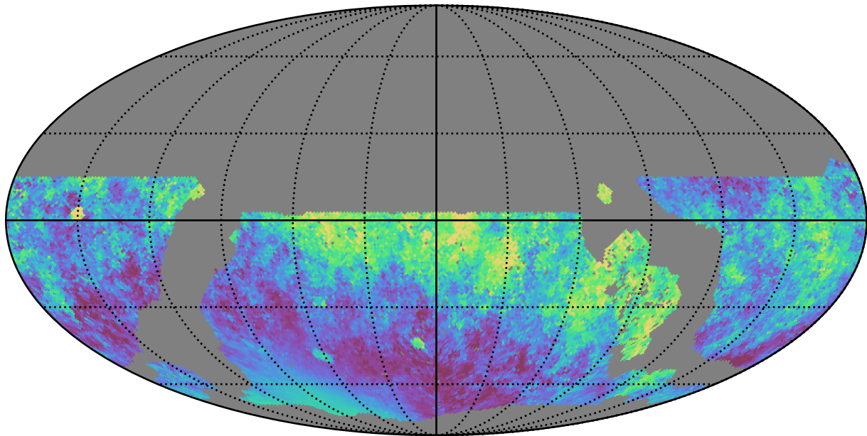
noroll_mjdp0_v3.4_10yrs WFD all bands: Median moonDistance
