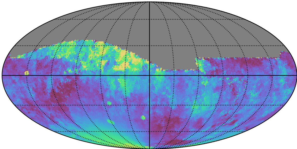
noroll_mjdp0_v3.4_10yrs All sky z band: Median moonDistance
