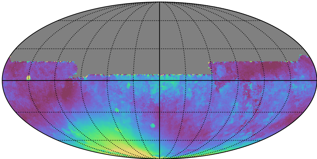
noroll_mjdp0_v3.4_10yrs All sky y band: Median moonDistance
