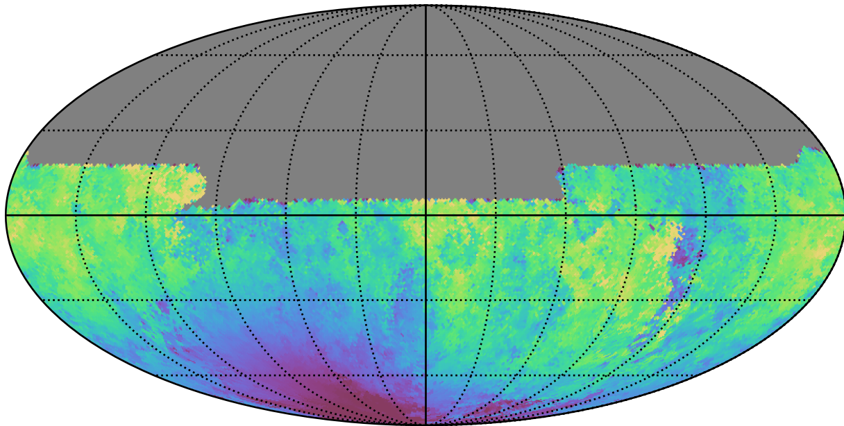
noroll_mjdp0_v3.4_10yrs All sky u band: Median moonDistance
