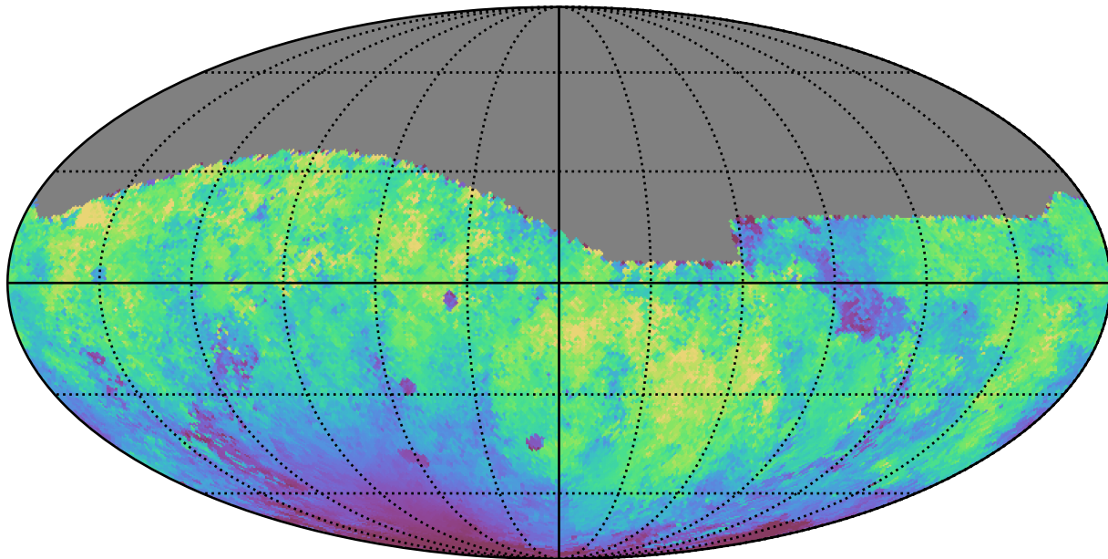
noroll_mjdp0_v3.4_10yrs All sky g band: Median moonDistance
