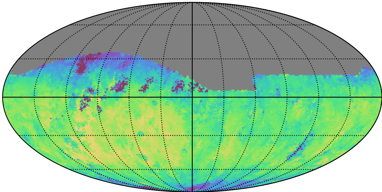
noroll_mjdp0_v3.4_10yrs Yr 1 r band: Median fiveSigmaDepth
