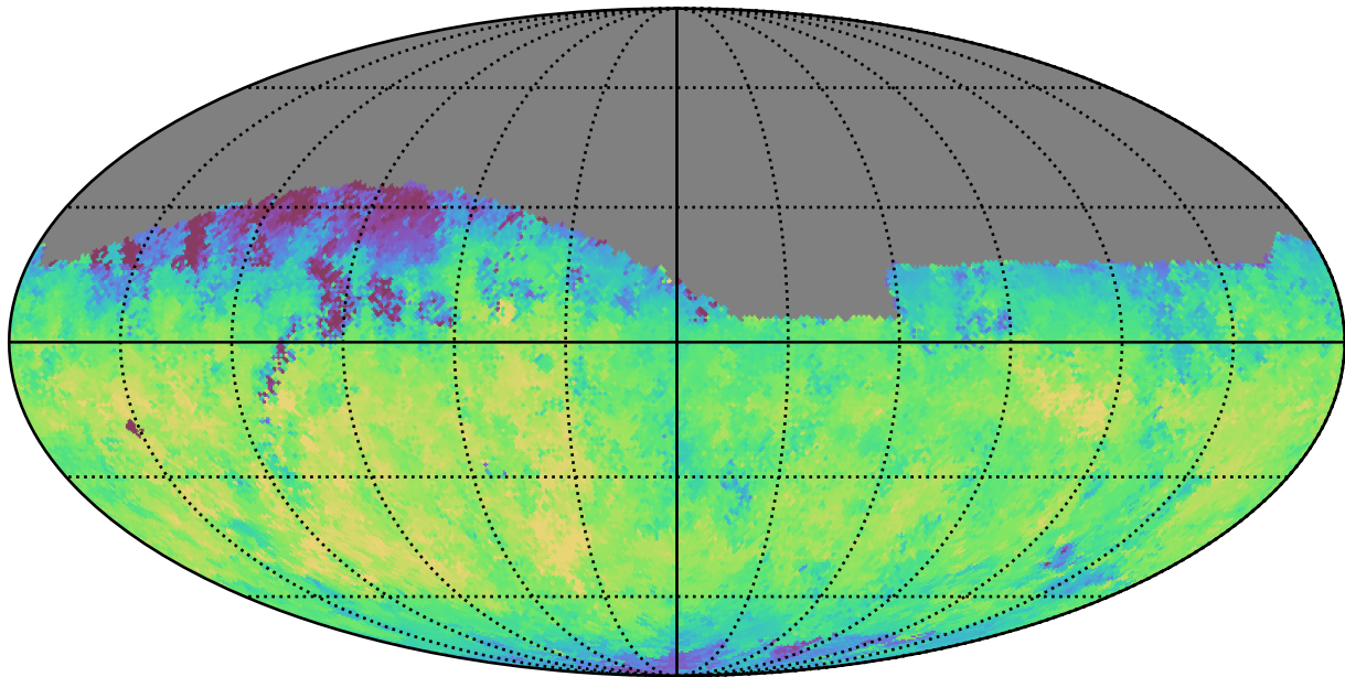
noroll_mjdp0_v3.4_10yrs Yr 1 i band: Median fiveSigmaDepth
