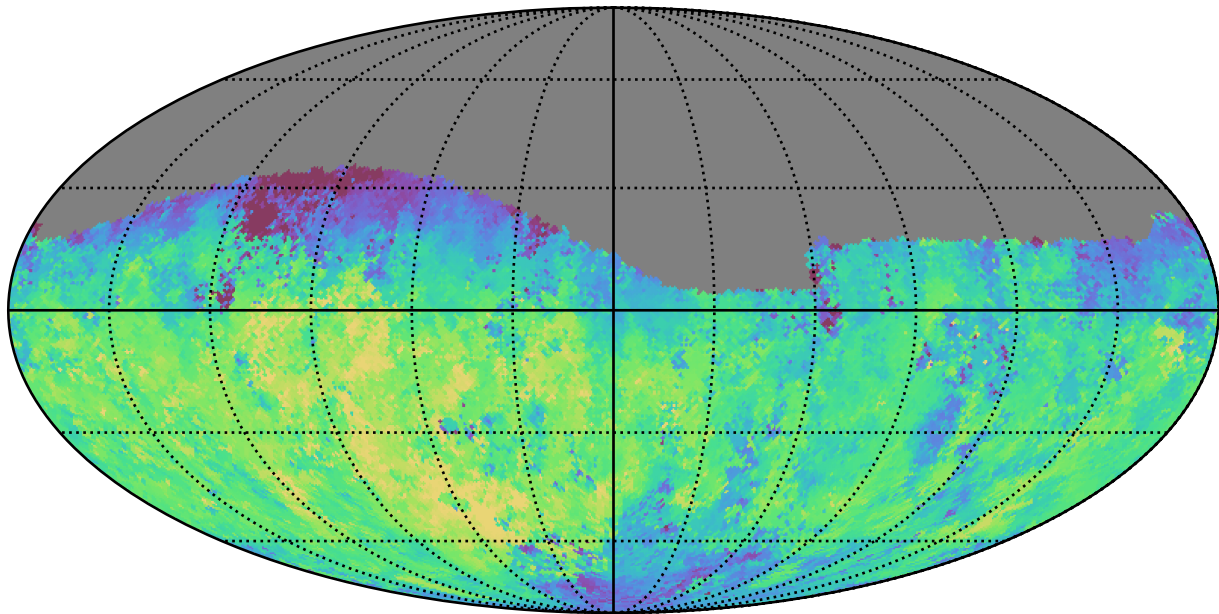
noroll_mjdp0_v3.4_10yrs Yr 1 g band: Median fiveSigmaDepth
