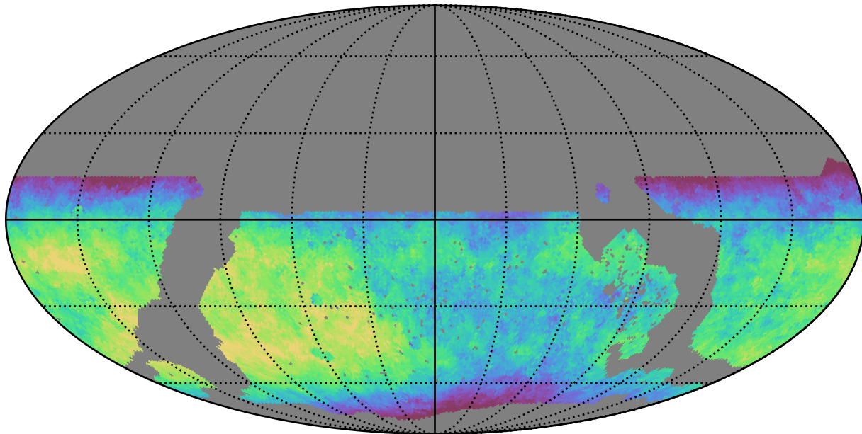
noroll_mjdp0_v3.4_10yrs WFD z band: Median fiveSigmaDepth
