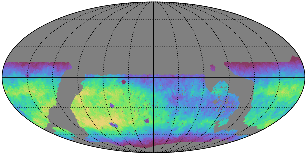
noroll_mjdp0_v3.4_10yrs WFD r band: Median fiveSigmaDepth
