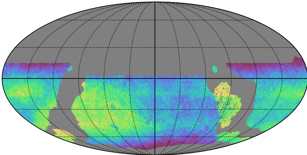
noroll_mjdp0_v3.4_10yrs WFD all bands: Median fiveSigmaDepth
