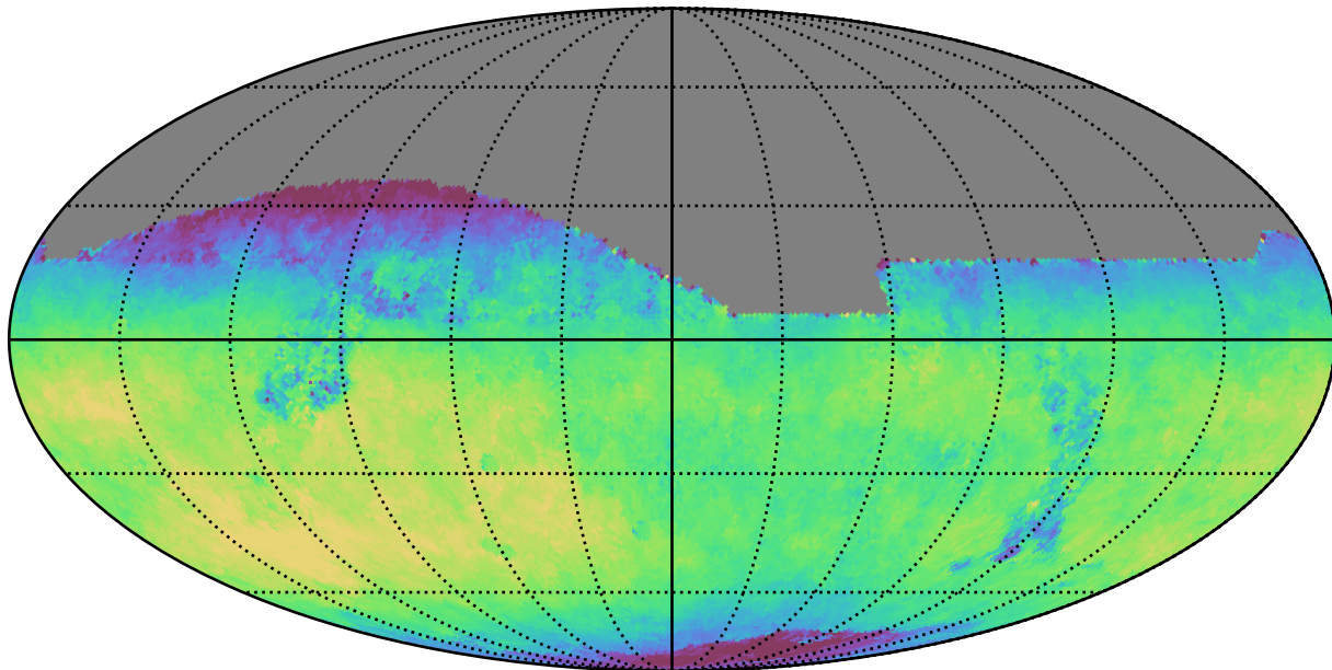
noroll_mjdp0_v3.4_10yrs All sky z band: Median fiveSigmaDepth
