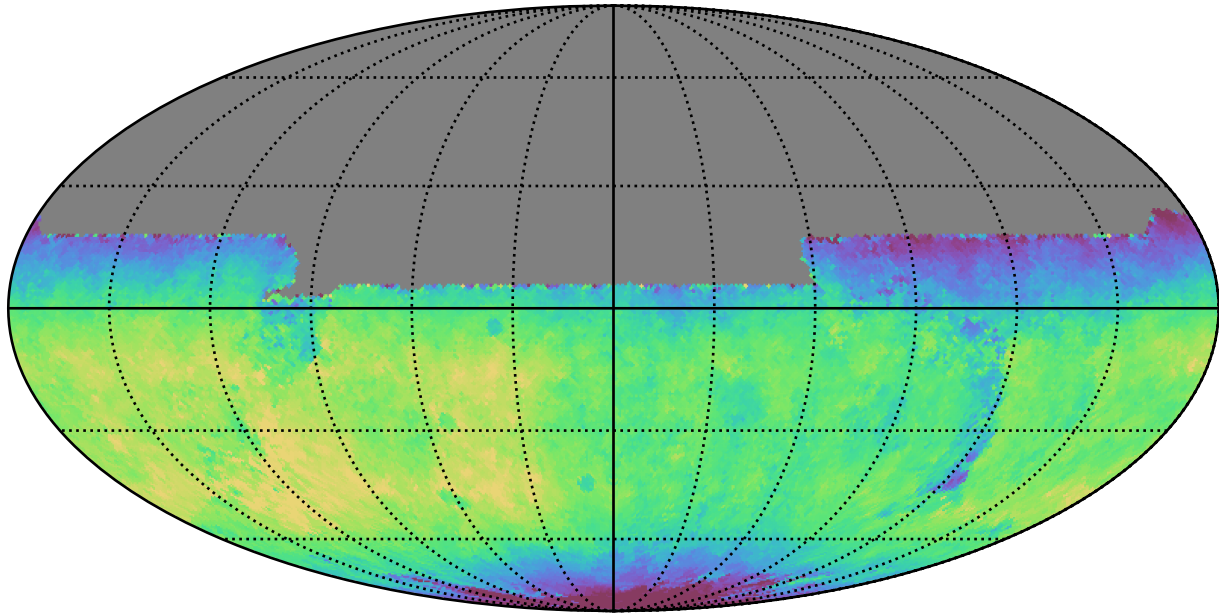
noroll_mjdp0_v3.4_10yrs All sky y band: Median fiveSigmaDepth
