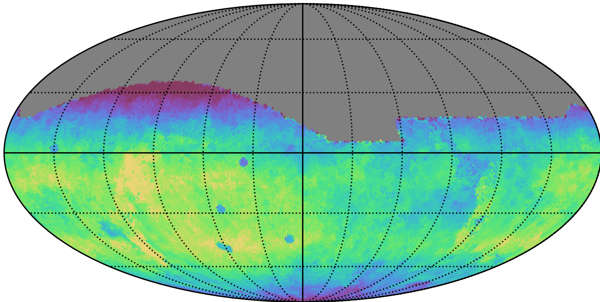
noroll_mjdp0_v3.4_10yrs All sky g band: Median fiveSigmaDepth
