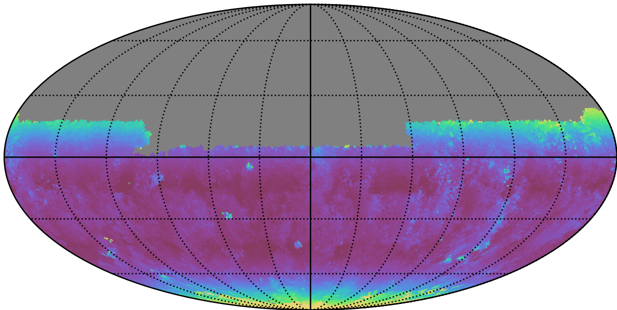
noroll_mjdp0_v3.4_10yrs Yr 1 y band: Median airmass
