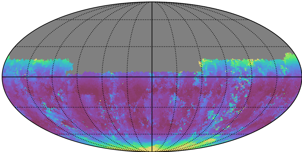
noroll_mjdp0_v3.4_10yrs Yr 1 u band: Median airmass
