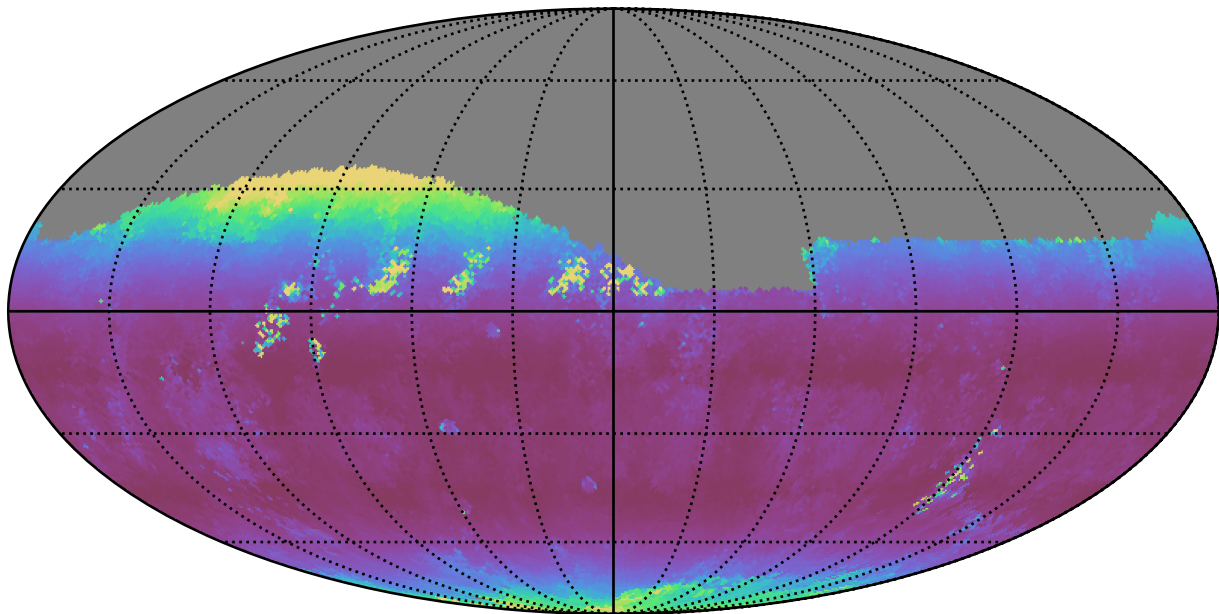
noroll_mjdp0_v3.4_10yrs Yr 1 r band: Median airmass
