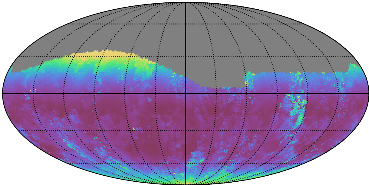
noroll_mjdp0_v3.4_10yrs Yr 1 g band: Median airmass
