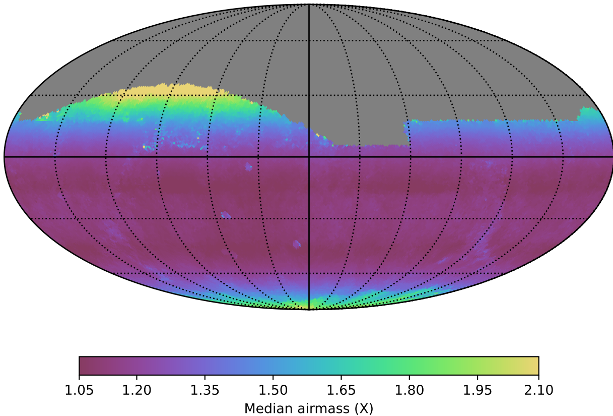
noroll_mjdp0_v3.4_10yrs Yr 1 all bands: Median airmass
