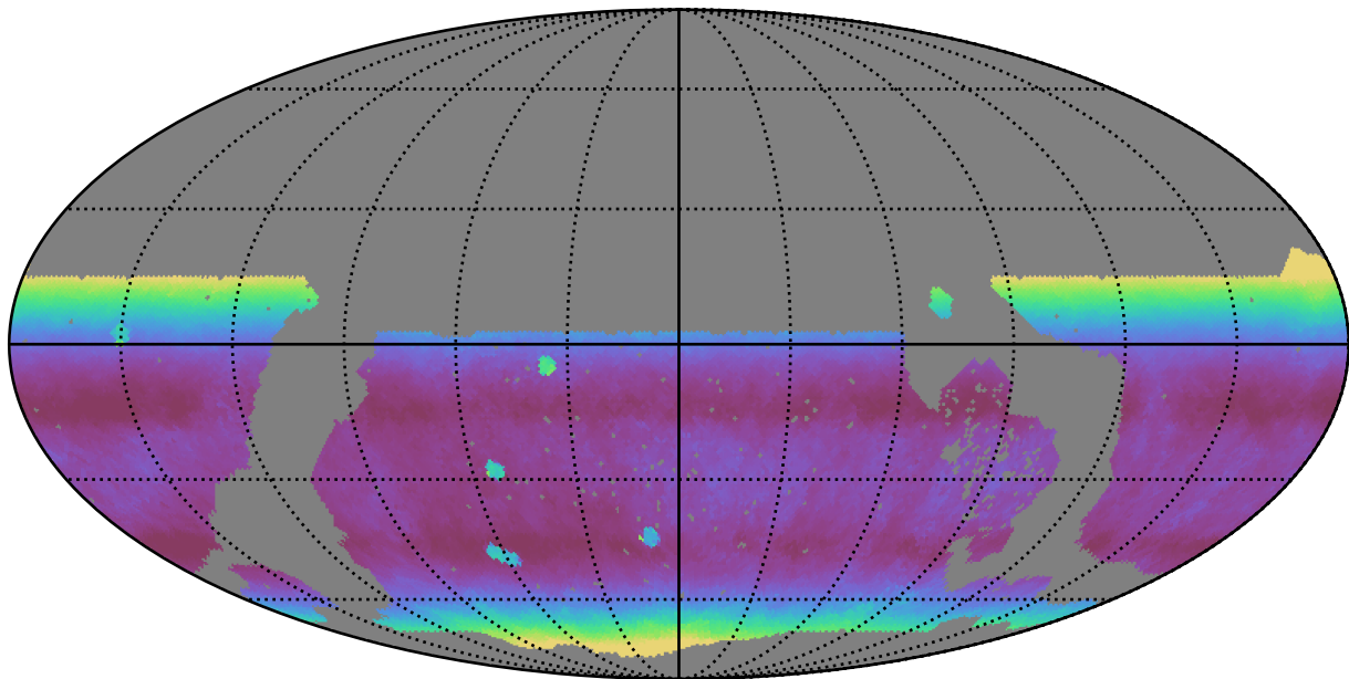
noroll_mjdp0_v3.4_10yrs WFD z band: Median airmass
