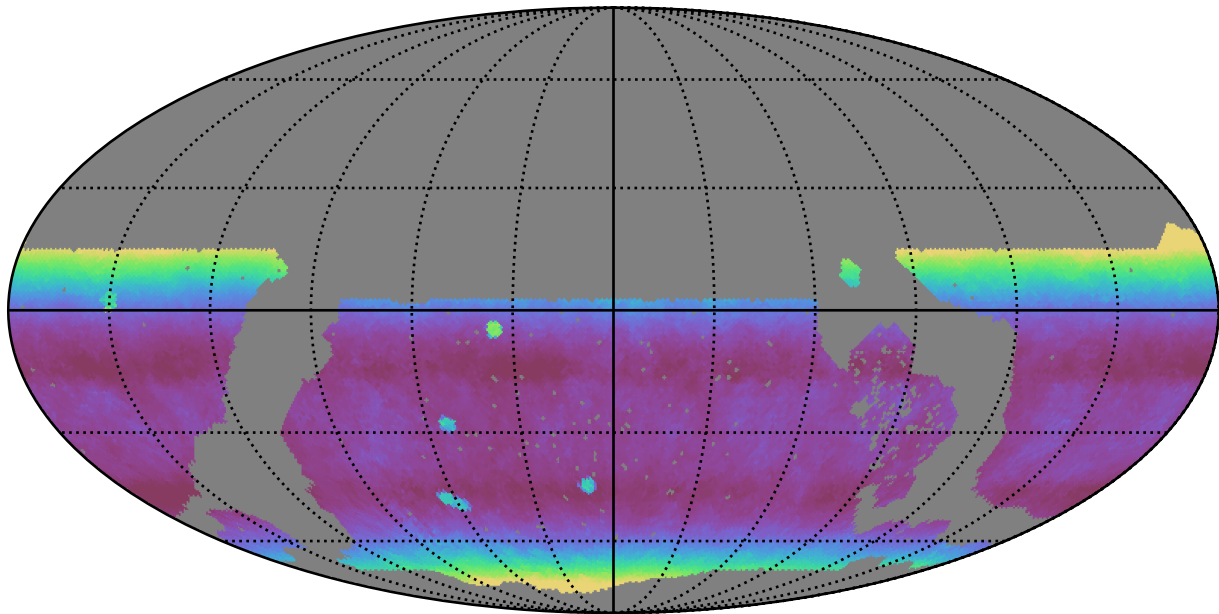
noroll_mjdp0_v3.4_10yrs WFD y band: Median airmass
