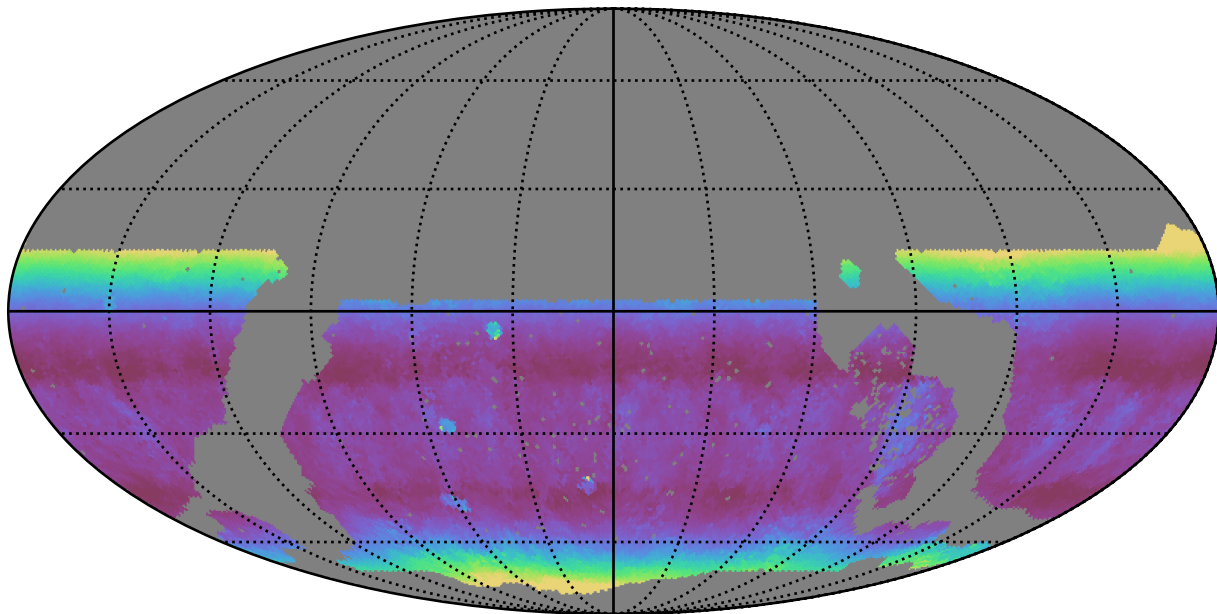
noroll_mjdp0_v3.4_10yrs WFD u band: Median airmass
