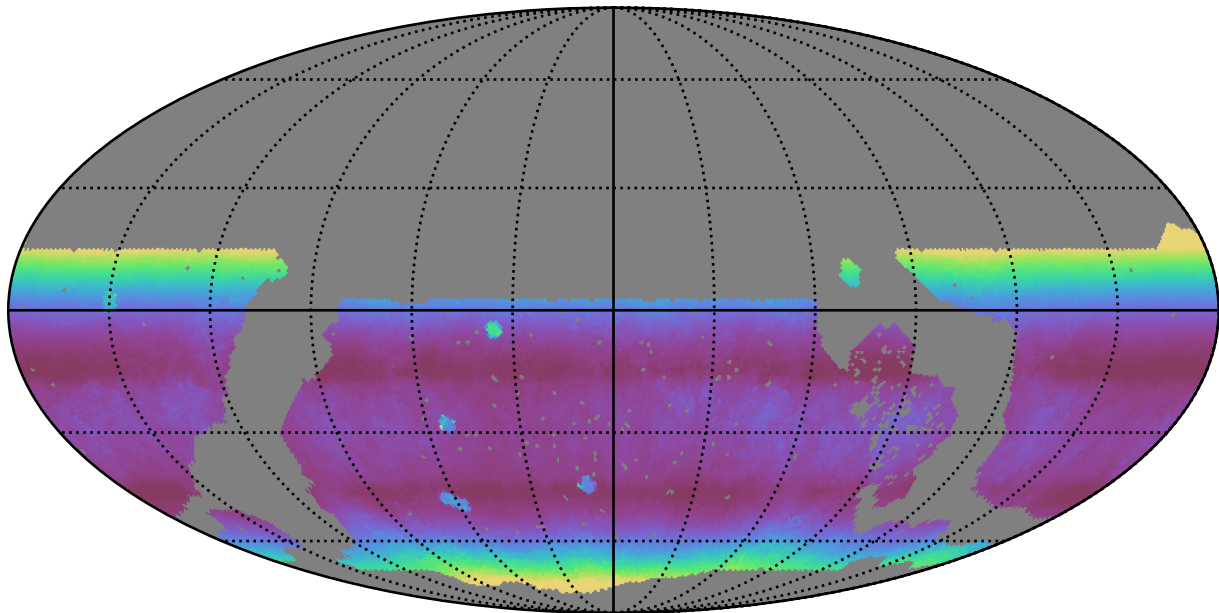
noroll_mjdp0_v3.4_10yrs WFD r band: Median airmass
