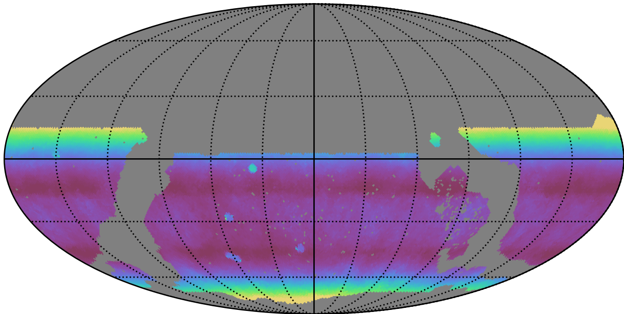
noroll_mjdp0_v3.4_10yrs WFD i band: Median airmass
