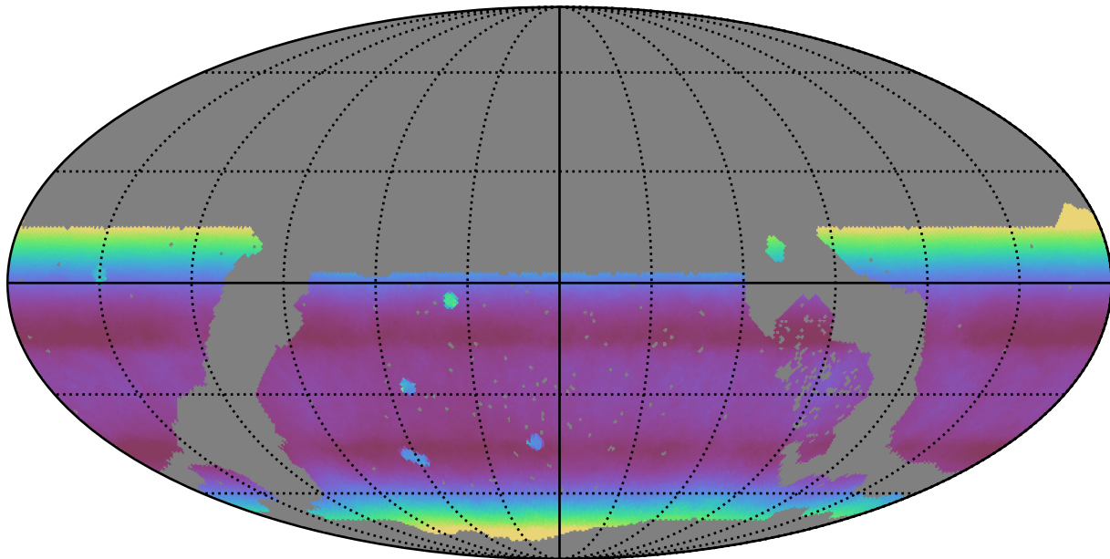
noroll_mjdp0_v3.4_10yrs WFD all bands: Median airmass
