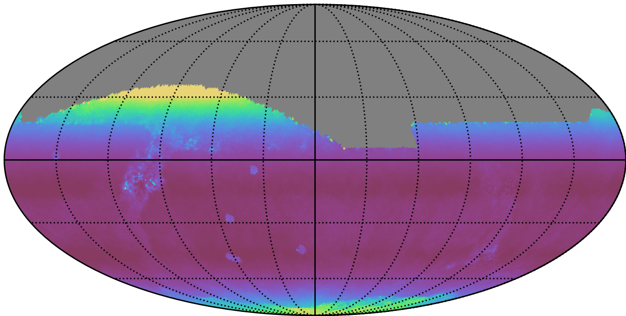
noroll_mjdp0_v3.4_10yrs All sky z band: Median airmass
