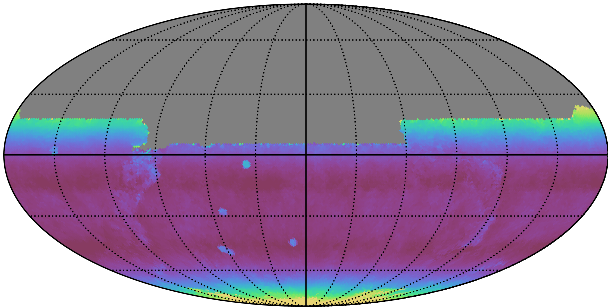
noroll_mjdp0_v3.4_10yrs All sky y band: Median airmass
