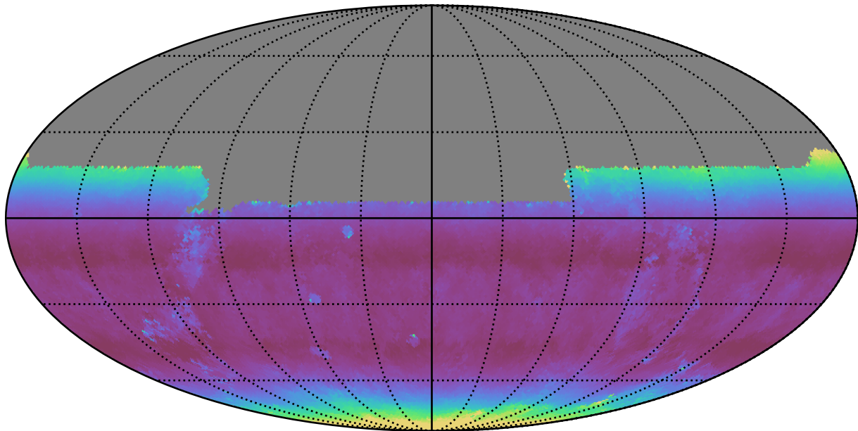
noroll_mjdp0_v3.4_10yrs All sky u band: Median airmass
