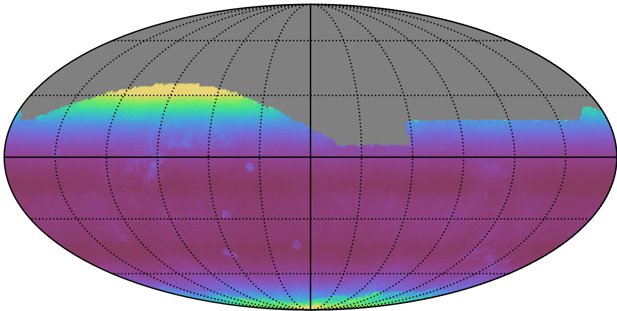
noroll_mjdp0_v3.4_10yrs All sky r band: Median airmass
