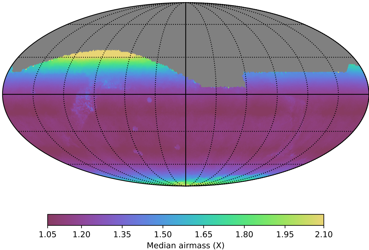
noroll_mjdp0_v3.4_10yrs All sky i band: Median airmass
