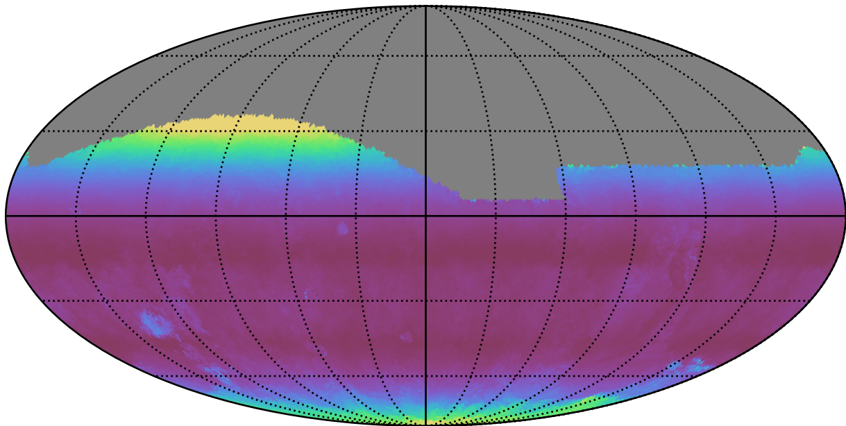
noroll_mjdp0_v3.4_10yrs All sky g band: Median airmass
