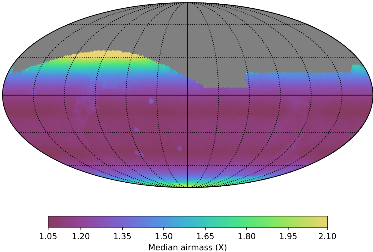
noroll_mjdp0_v3.4_10yrs All sky all bands: Median airmass
