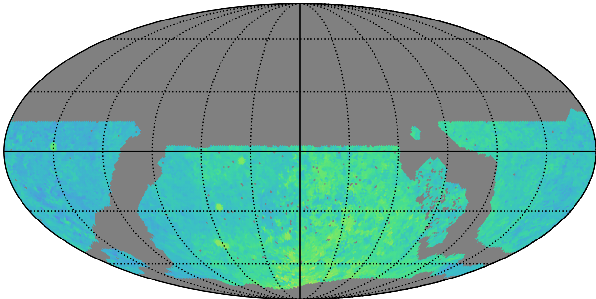
noroll_mjdp0_v3.4_10yrs WFD z band: Median Season Length
