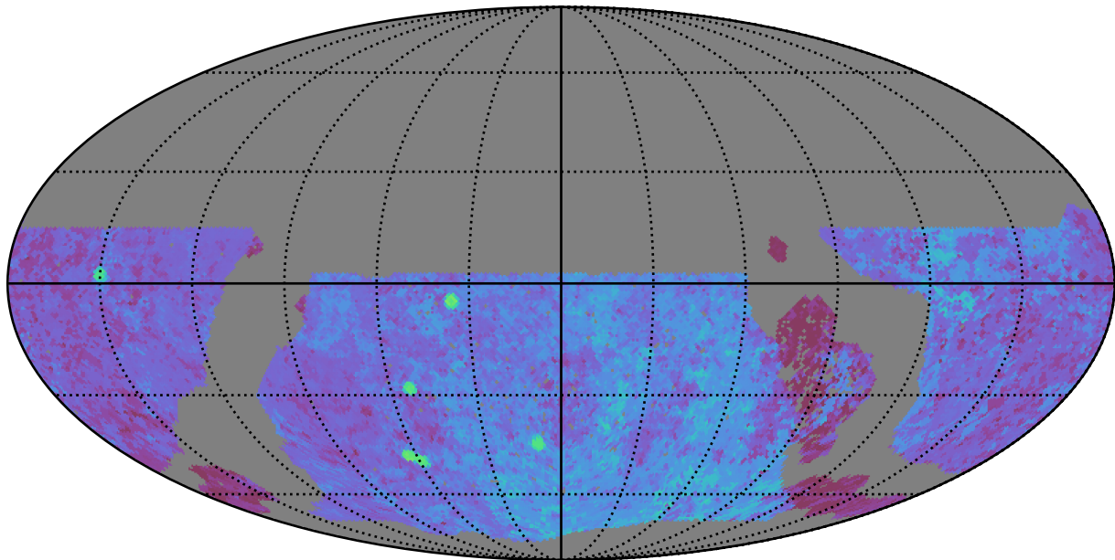
noroll_mjdp0_v3.4_10yrs WFD u band: Median Season Length
