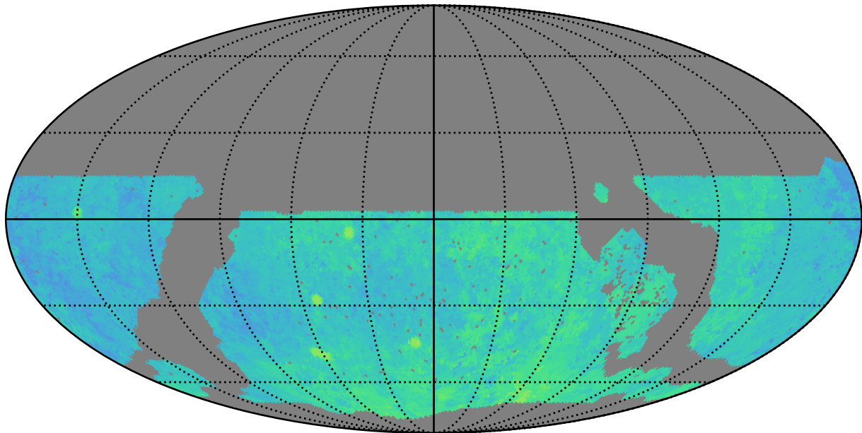
noroll_mjdp0_v3.4_10yrs WFD r band: Median Season Length
