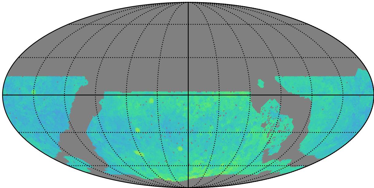
noroll_mjdp0_v3.4_10yrs WFD i band: Median Season Length
